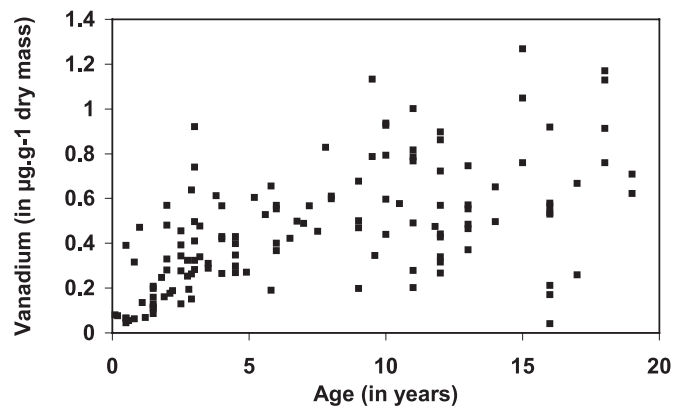
Fig. 4. Concentrations of vanadium ( \mu\text{g g}^{-1} dry mass) in the kidney (upper frame) and the liver (lower frame) of the common dolphin, Delphinus delphis , of the Bay of Biscay as a function of the age.
